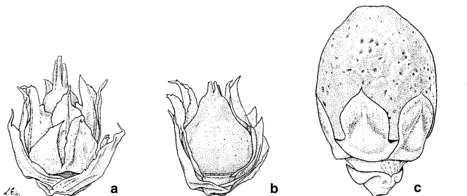
Fig. 1. Female spikelets in fruiting stage, a–b , H. humilis , a , as dispersed, nut surrounded by tepals, floral bracts and spikelet bracts; b , as (a) but some bracts and tepals removed (48 km SW of Ravensthorpe, Briggs 460 NSW); c , H. pubescens , as dispersed, nut with tepals and floral bracts (10 km WNW of Busselton, Briggs 6463 NSW). Scale bar = 2 mm.
