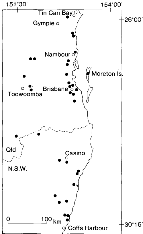
Fig. 8. Distribution of A. woodsiana .
